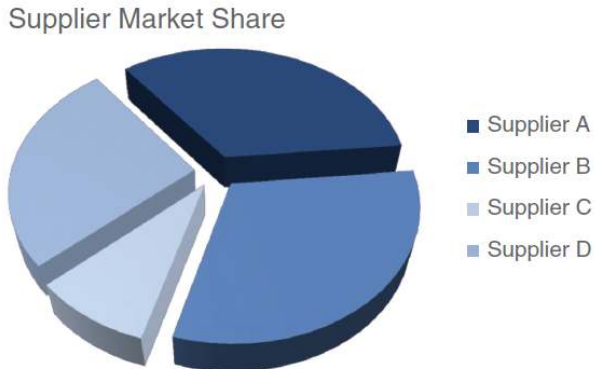
FIGURE 2.21 Pie chart
