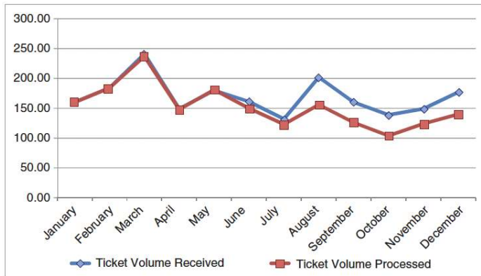
FIGURE 3.17 Original graph
