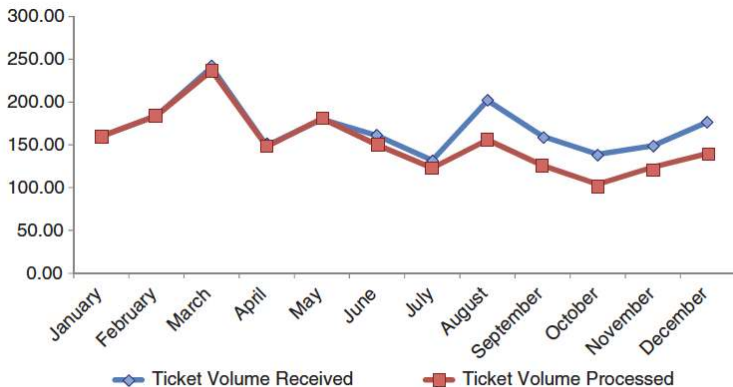
FIGURE 3.19 Remove gridlines
