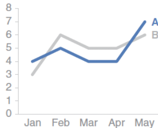
FIGURE 2.8 Line graphs
